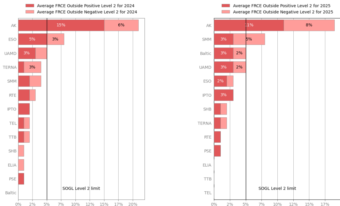
Figure 6.2 Percentage of time average FRCE was outside level 2 targets for 2024 and 2025
