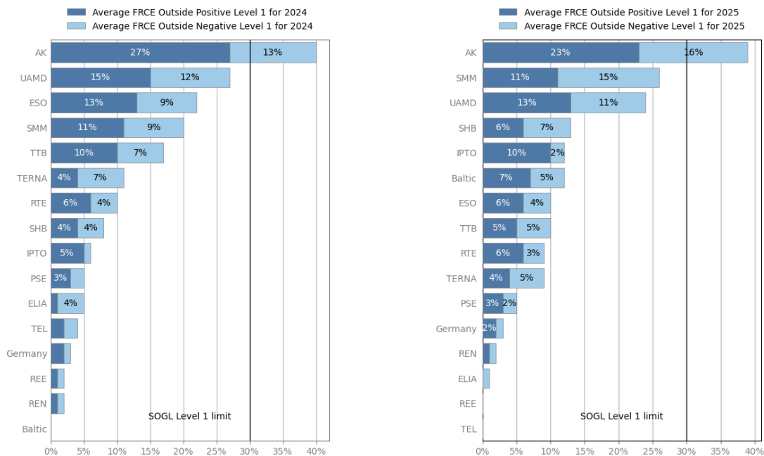
Figure 6.1 Percentage of time average FRCE was outside level 1 targets for 2024 and 2025
