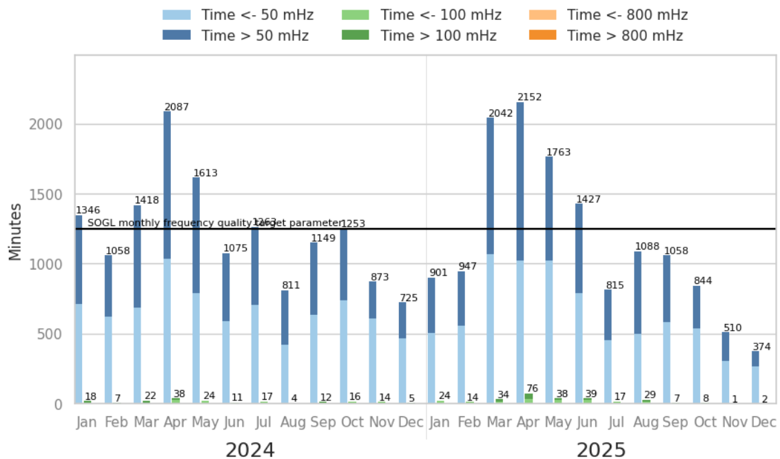
Figure 5 Monthly number of minutes outside the standard ranges in Continental Europe for 2024 and 2025
