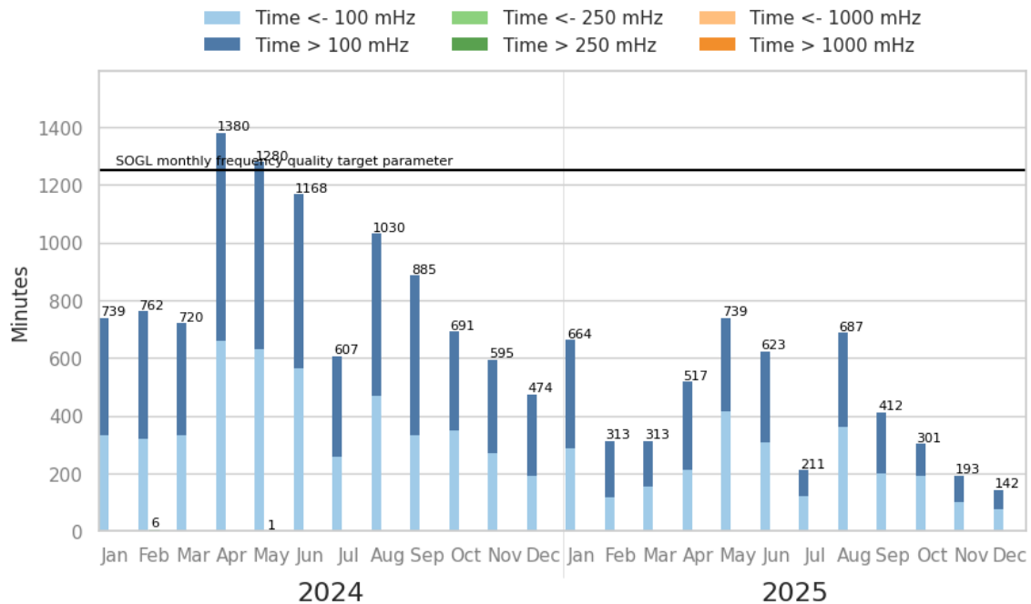
Figure 20 Monthly number of minutes outside the standard ranges in the Nordic synchronous area for 2024 and 2025
