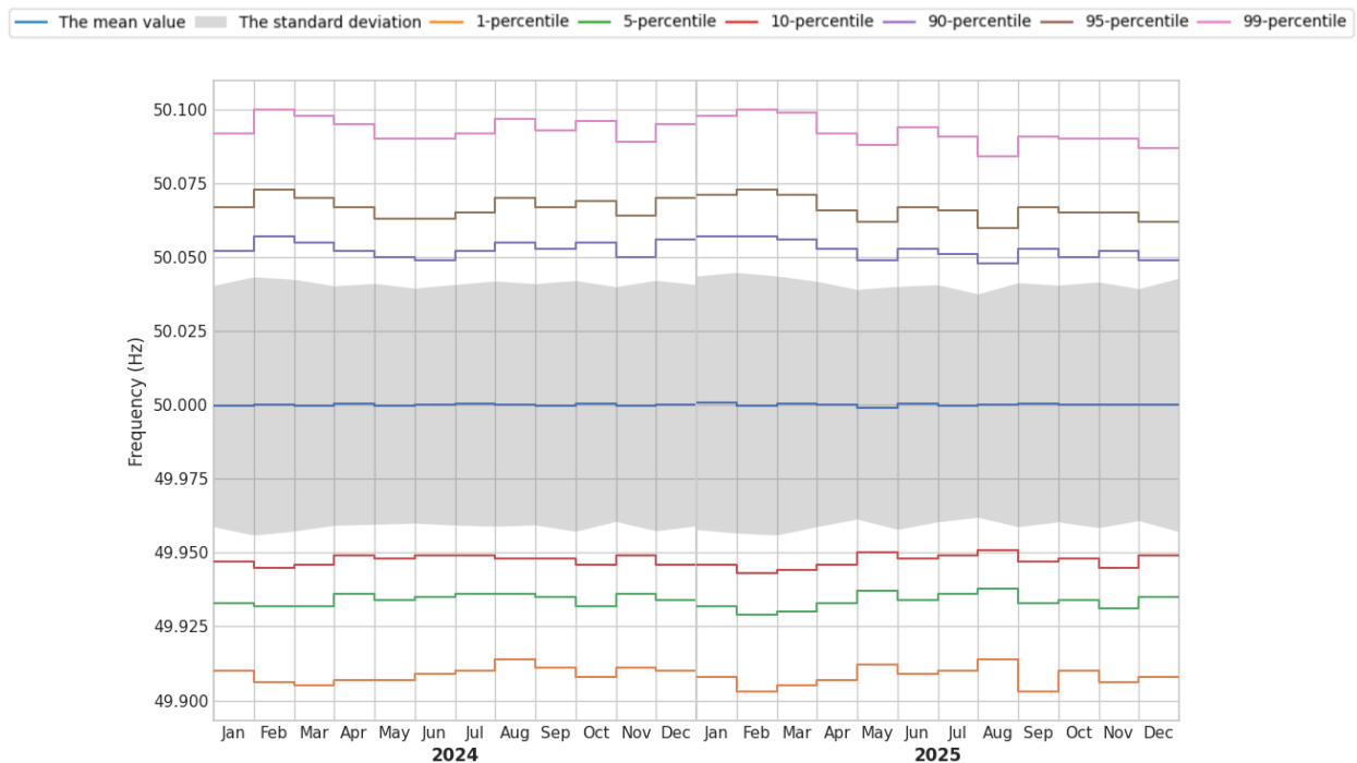
Figure 14 Monthly frequency percentiles and standard deviation in Ireland/Northern Ireland 2024 and 2025
