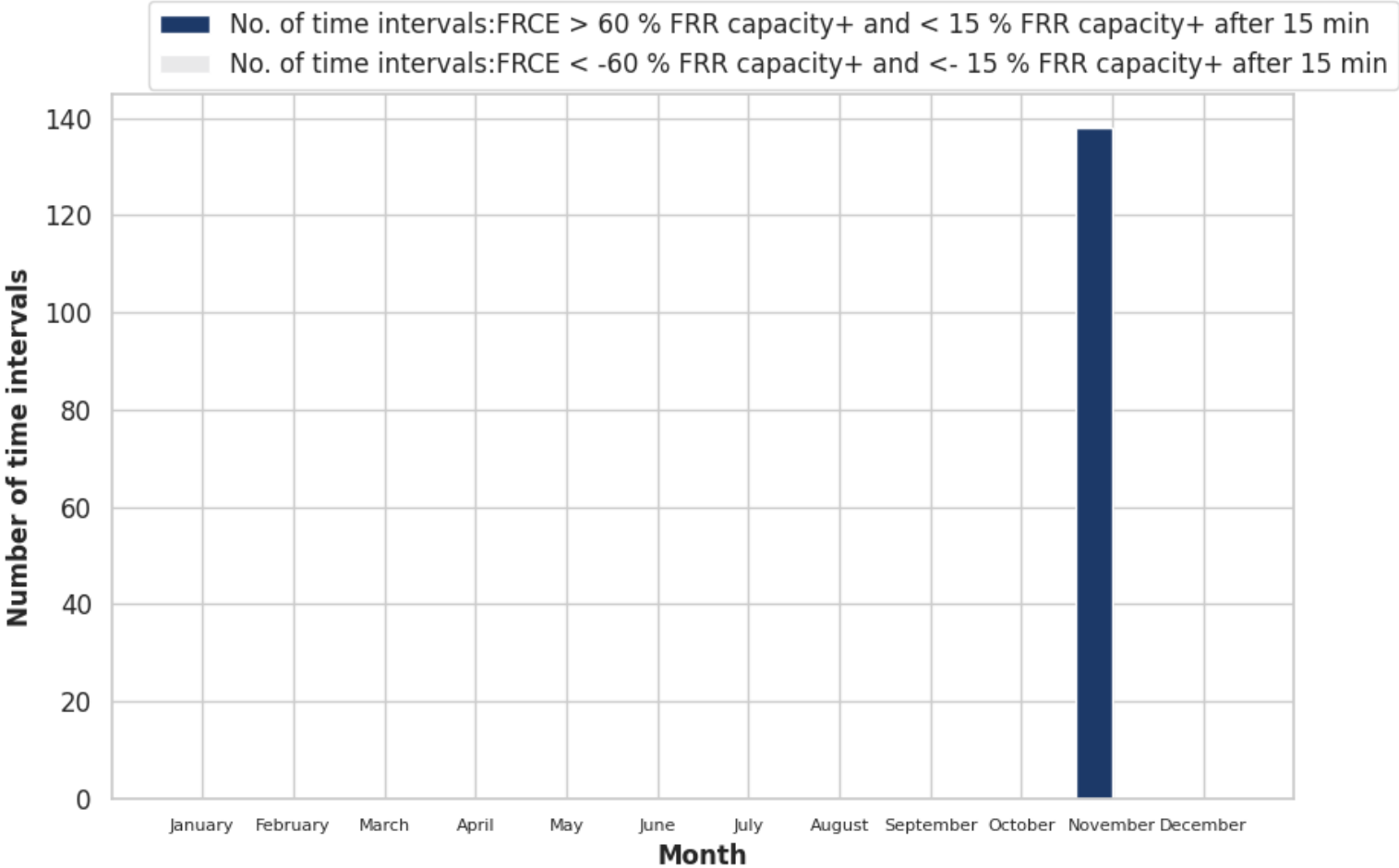
Figure 25 Nordic LFC 2024 FRCE Outside FRR Capacity within 15 minutes
